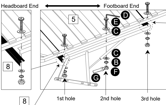
8 Metal horizontal support bar
