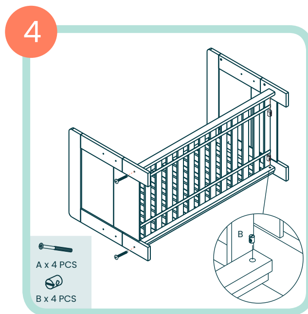
Assemble mattress to cot end using 4 x A bolts and 4 x B nuts
